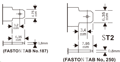
Typical View of Female insert Terminal.
